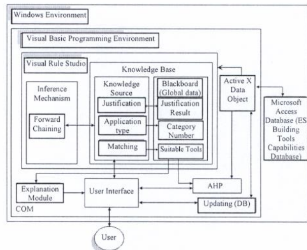
Figure 3. Blackboard architecture of the proposed expert system.
