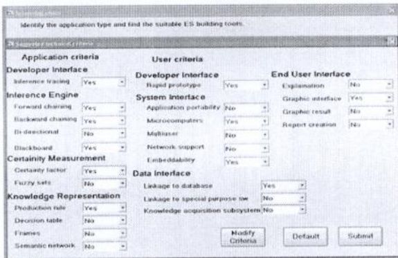
Figure 8. A sample of screenshots during screening phase.
