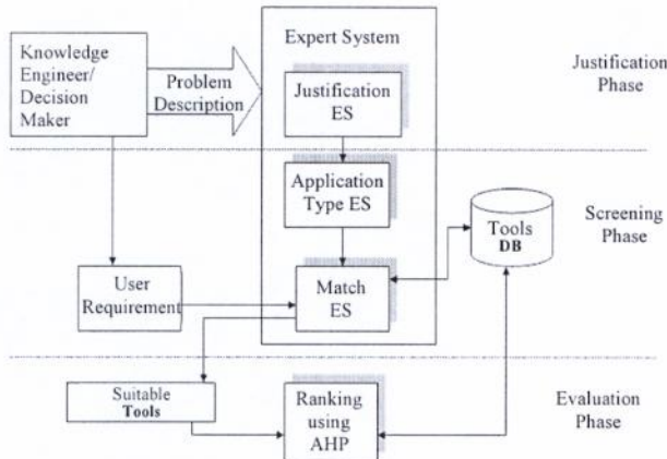
Figure 1. Framework of the proposed approach.
