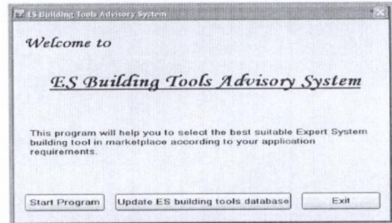
Figure 5. Main screen.
