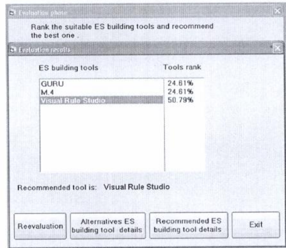
Figure 11. Output of the evaluation phase.
